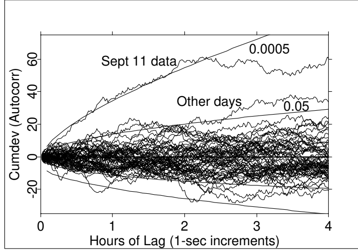
Fig. 4. Cumulative deviation of autocorrelation of the device variance. The cumulative sum is shown as a function of lag time for September 11, 2001, contrasted with the same calculation for 60 surrounding days. The autocorrelations were calculated for 24 hour EDT days over lags of up to four hours.
