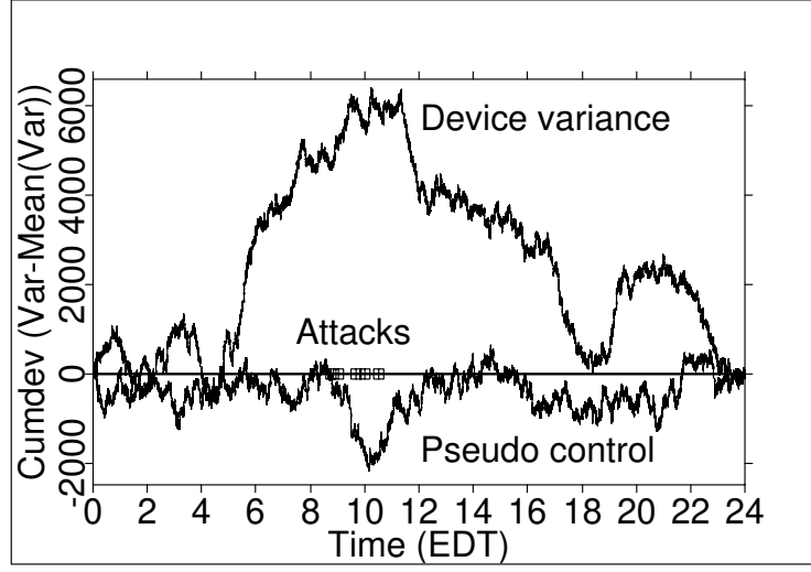
Fig. 3. Cumulative deviation of device variance across RNG nodes, relative to the empirical mean value, for each second on September 11, 2001. The truly random data from the RNG array are contrasted with a pseudo-random control dataset computed for the same array of data elements processed with the same algorithms. Axis labeling is in EDT. Times of the terrorist attacks are indicated with boxes on the zero line.
