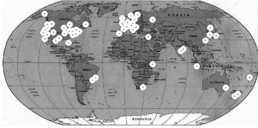
Fig. 1. Locations of host sites for the RNG nodes. Distribution is opportunistic because the network depends on voluntary collaboration.
