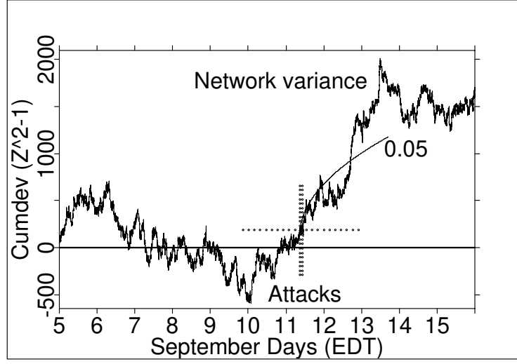
Fig. 2. Cumulative deviation of network variance for each second, September 5 through 15, 2001. Day boundaries are in Eastern Daylight Time (EDT). The terrorist attacks are marked with a pair of vertical dotted lines at 08:45 and 10:30 on September 11. A segment of a parabolic envelope of 5% probability with its origin at the level of the random walk at 08:45 (horizontal dotted line) provides scale for the persistent trend.
